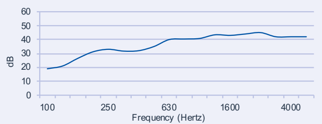
1/3 octave transmission loss Rw 40 door
