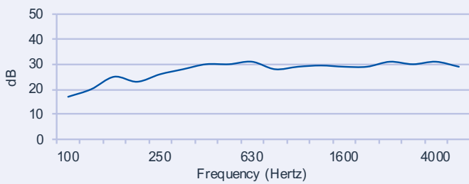
1/3 octave transmission loss Rw 35 door
