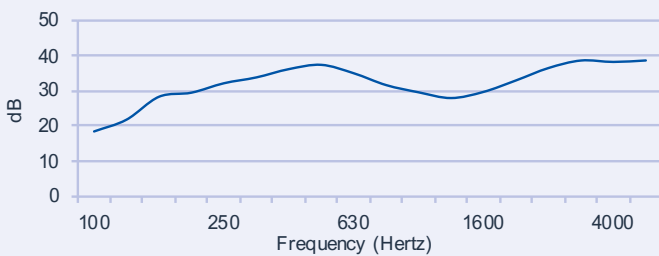
1/3 octave transmission loss Rw 35 door
