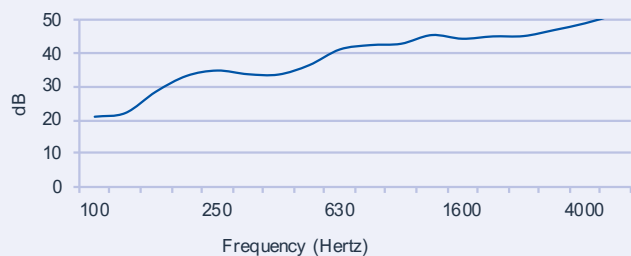
1/3 octave transmission loss Rw 41 door
