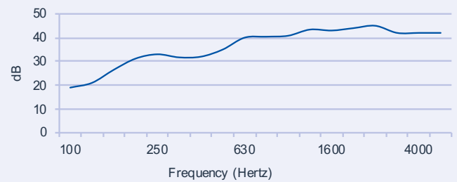
1/3 octave transmission loss Rw 45 door
