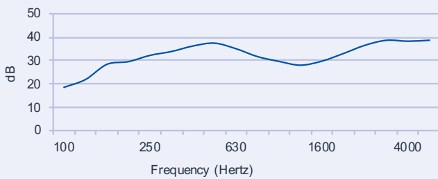
1/3 octave transmission loss Rw 41 door
